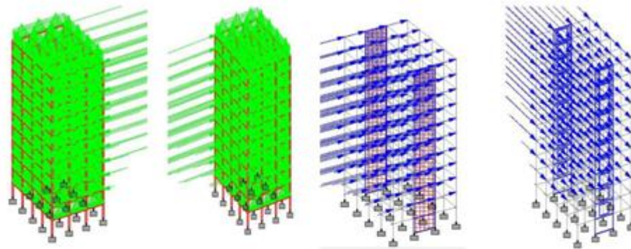
Load Combination along Positive- X direction for Model 1
