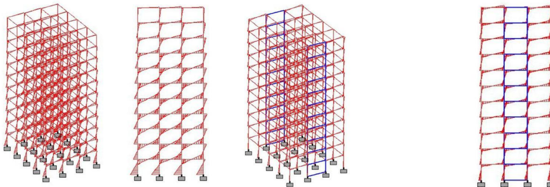
Figure 10:- Maximum Bending Moment
